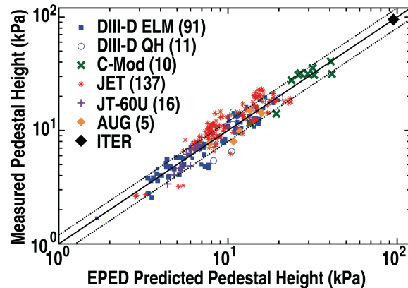
Figure 1: (a) Typical structure of a peeling-ballooning mode in the DIII-D tokamak, calculated by ELITE. (b) Comparison of pedestal height predicted by the EPED model with observations on 5 tokamaks, with a prediction for ITER also shown.
