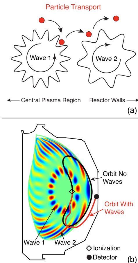
Figure 1: (a) Cartoon showing influence of one wave on the losses caused by another. (b) Similar situation for losses induced by two different waves in a fusion device and how those particles can hit a detector to designed to measure them.
