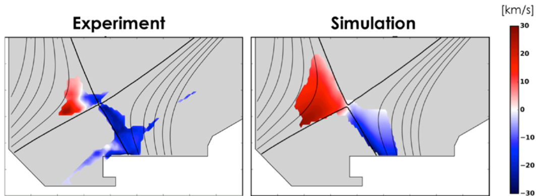
Figure 2: Measured and simulated helium ion velocity the lower divertor of a DIII-D plasmas. Both the experiment and the numerical simulation display similar velocity magnitude and direction. Images courtesy of LLNL.
