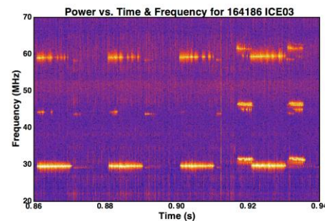
Figure 1: The top image is an example of raw data the team captured at DIII-D showing fluctuations in the magnetic field. An equation known as a Fourier Transform was used to plot the frequency and duration of individual waves, represented by the orange bars in the bottom image. Courtesy of DIII-D National Fusion Facility.
